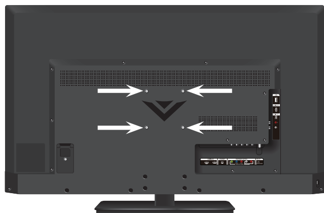
E400i-B2 - WALL MOUNT SCREW LOCATIONS
