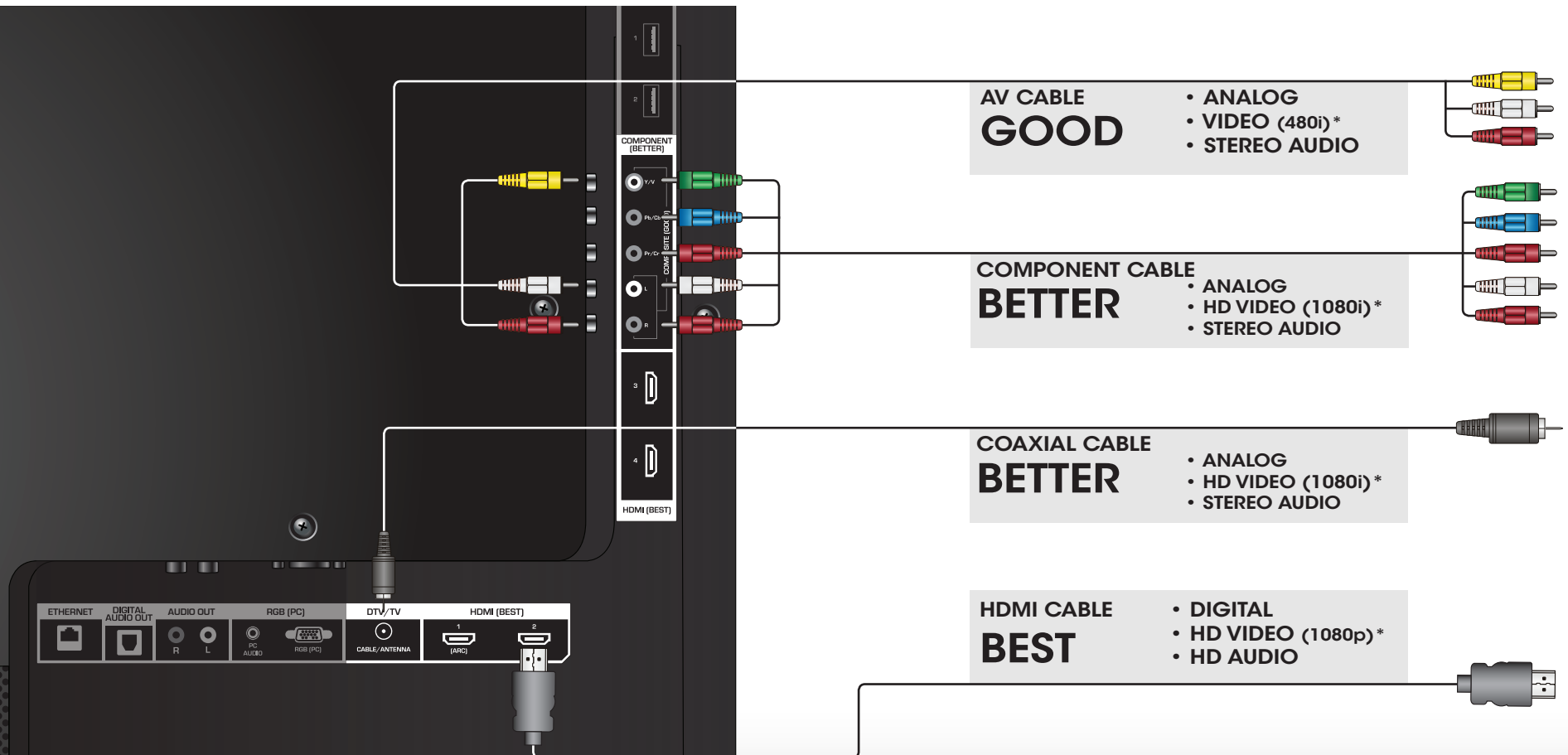
DVD/Blu-ray Player
