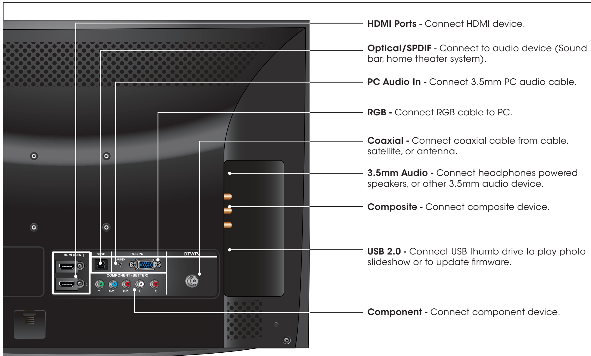
Rear Panel - E261VA
