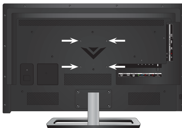
WALL-MOUNT SCREW LOCATIONS
