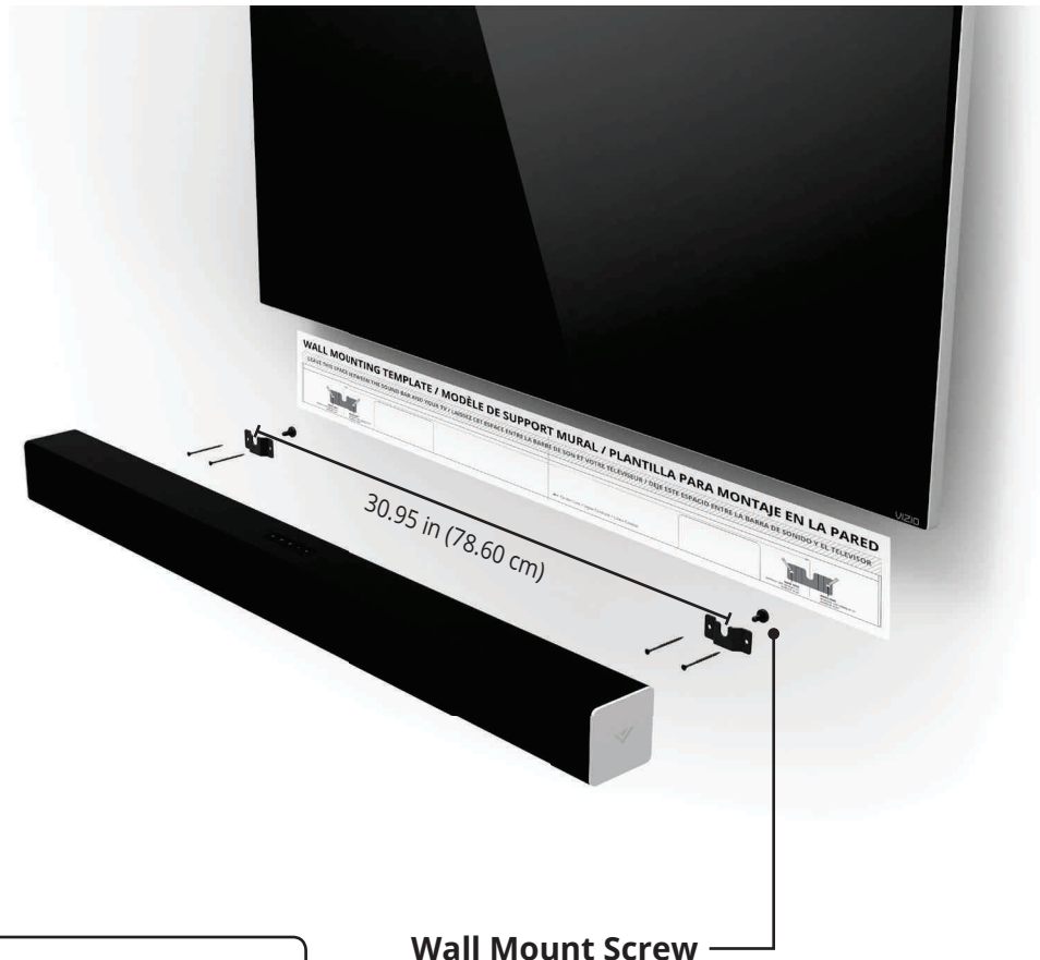
Wall Mount Screw Screw Size: M4 x 10
